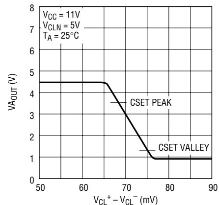
Current Limit Amplifier CA1 Gain at V_{CC} = 11\text{V} , V_{CL}^- = 5\text{V}
